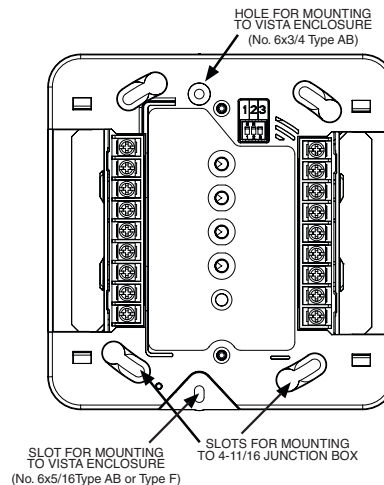
FIGURE 2: MOUNTING
