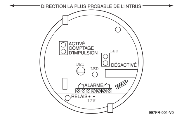
Figure 1. Orientation de montage optimale
