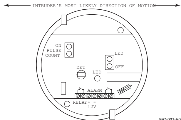
Figure 1. Optimum Mounting Orientation
