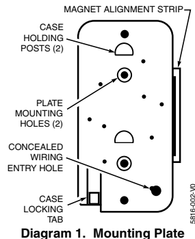
Diagram 1. Mounting Plate
