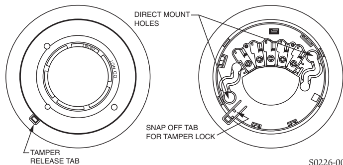
FIGURE 2: TAMPER-RESISTANT FEATURE
