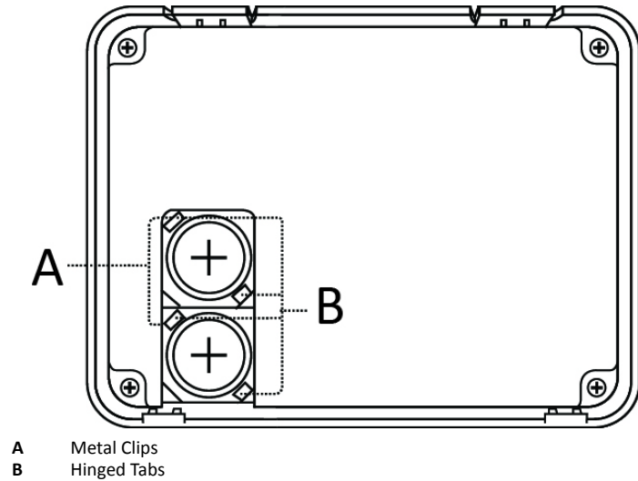
Figure 4 Wireless Keypad—Battery Compartment
